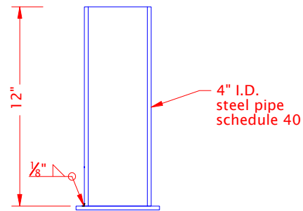
PIPE SLEEVE
