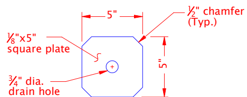
BASE PLATE BASE ASSEMBLY
