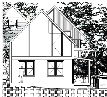
① HOUSE #3 N-S SECTION 1/4" = 1'-0"
