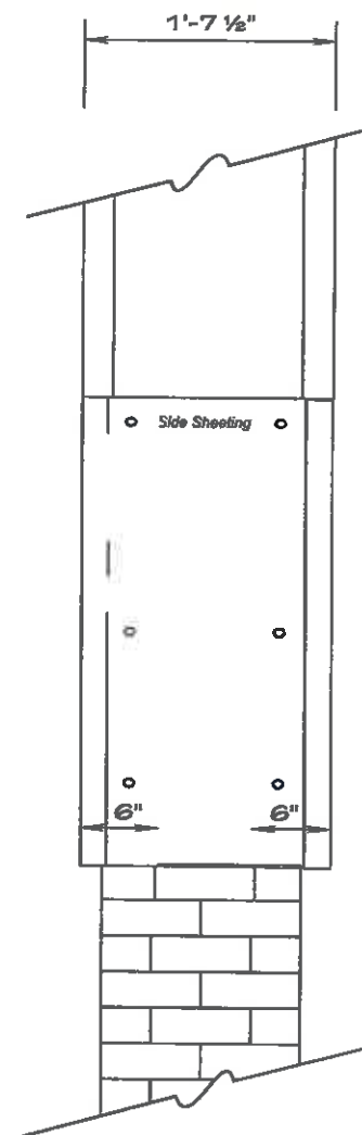
1.2 SIDE VIEW / DETAIL
