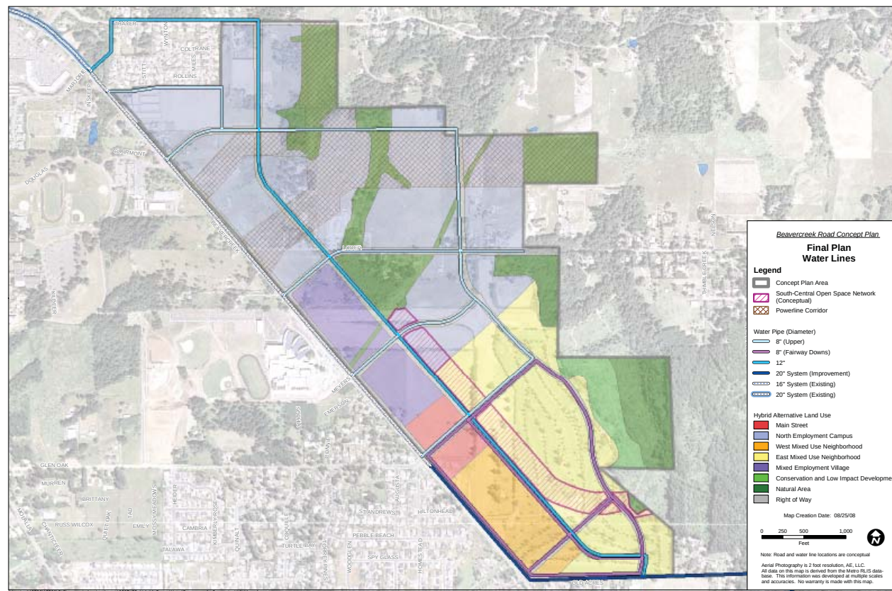
Figure 22 - Water Plan
