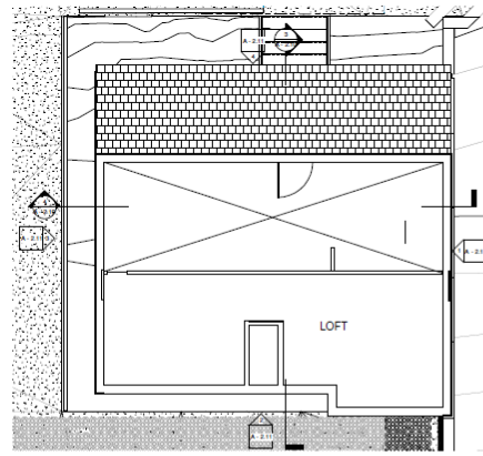
② HOUSE #1 LOFT 1/8" = 1'-0"
