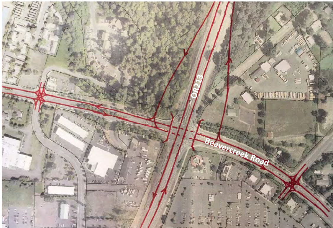
Exhibit 8 – Alternative 5: Half Diamond Interchange Alternative
