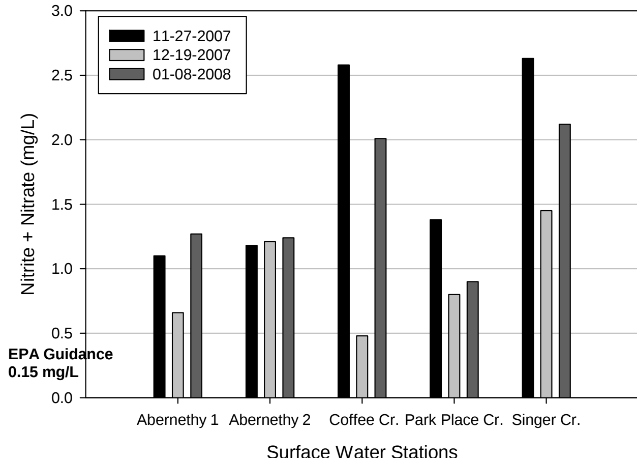
Figure 27. Nitrates—Stormwater Monitoring (2007–2008). Monitoring site locations are described in Appendix A
