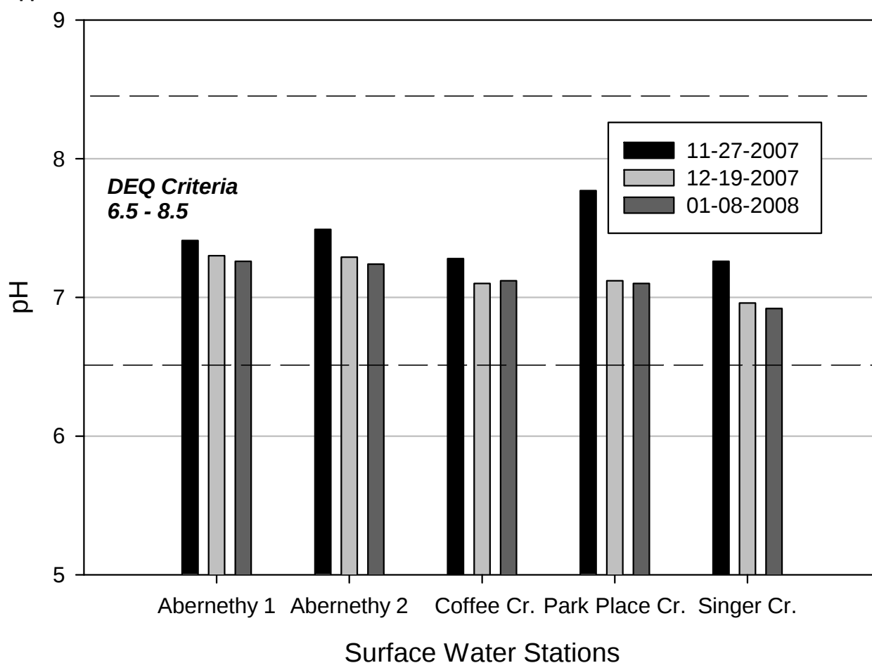
Figure 22. pH—Stormwater Monitoring (2007–2008). Monitoring site locations are described in Appendix A
