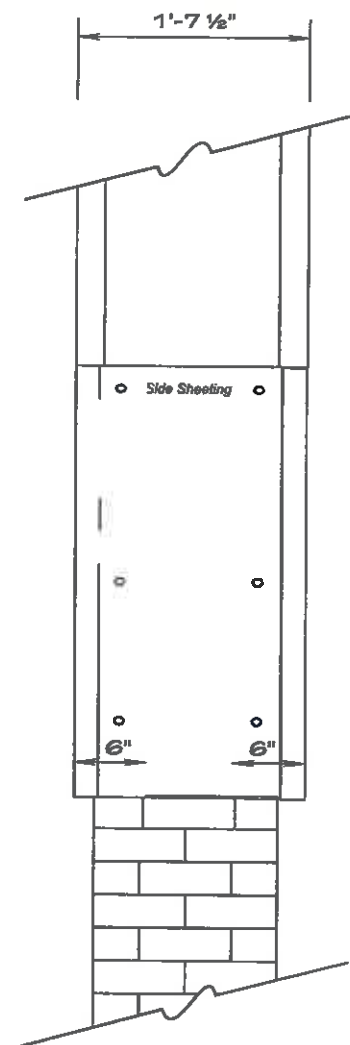
1.2 SIDE VIEW / DETAIL
